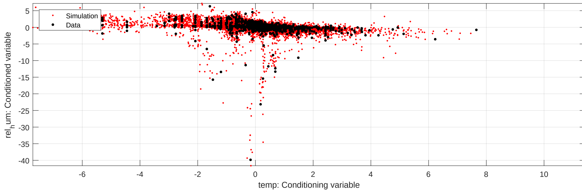
rel h um|temp: H&T simulation on Laplace margins
