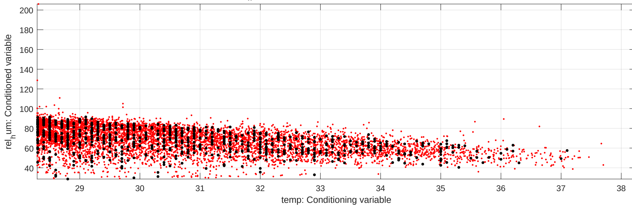
rel h um|temp: H&T simulation on original scale
